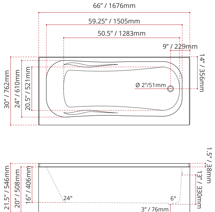
MODEL NUMBER : 4251 (RIGHT HAND DRAIN LOCATION)
