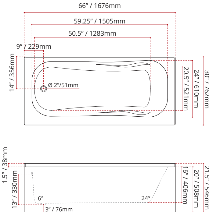
MODEL NUMBER : 4241 (LEFT HAND DRAIN LOCATION)
